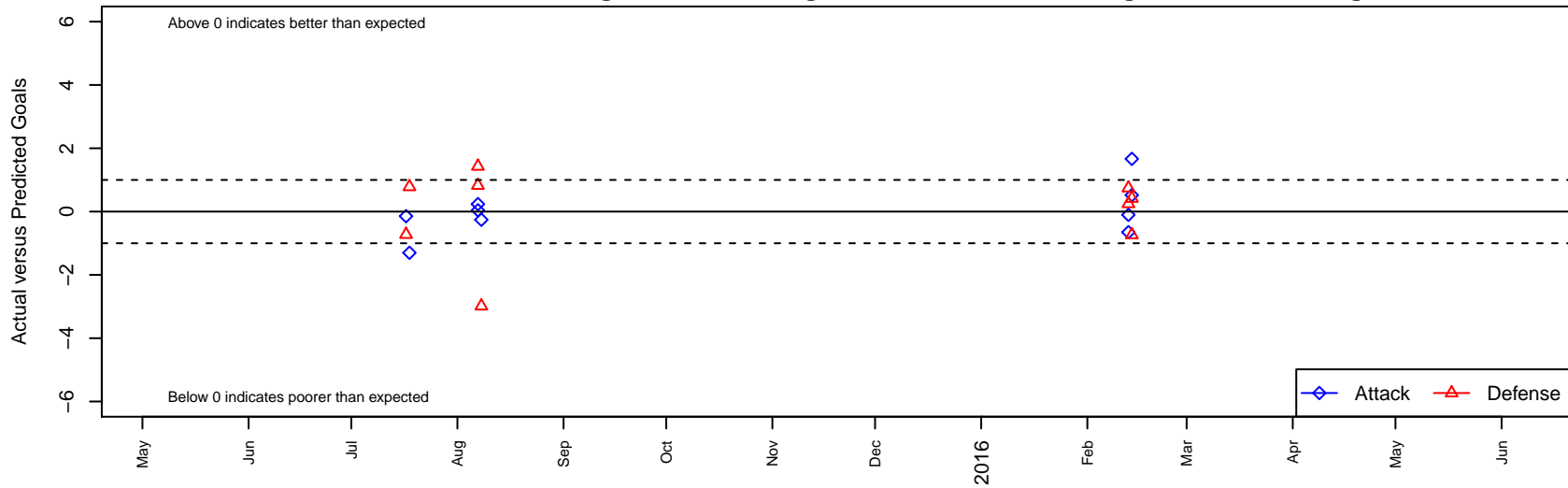
Folsom SC Force B98 Dots are actual minus expected GF (blue circles) and GA (red triangles). Blue line is smoothed change in attack strength. Red is smoothed change in defense strength.
